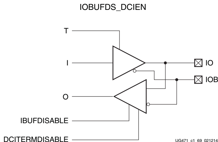
Figure 1-28: Differential Bidirectional Buffer With Input Path Disable and DCI Disable (IOBUFDS_DCIEN)
