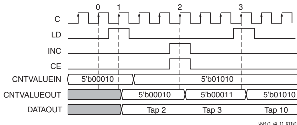
Figure 2-13: IDELAY in VAR_LOAD Timing Diagram
