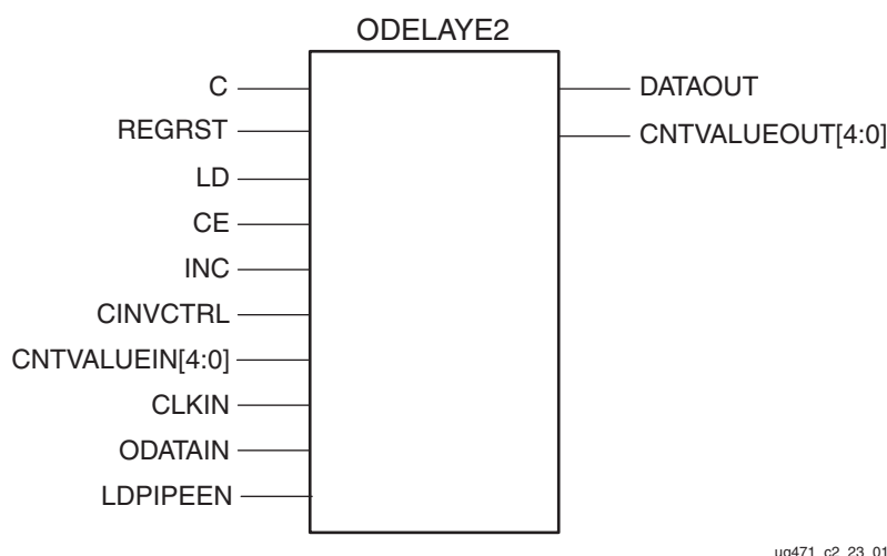
Figure 2-25: ODELAYE2 Primitive
