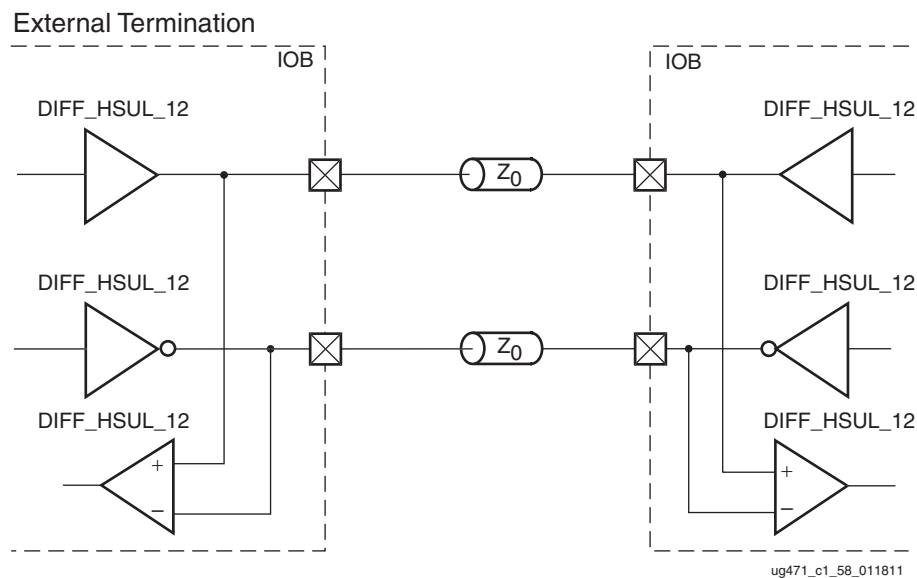
Figure 1-68: Differential HSUL_12 with Bidirectional Signalling
