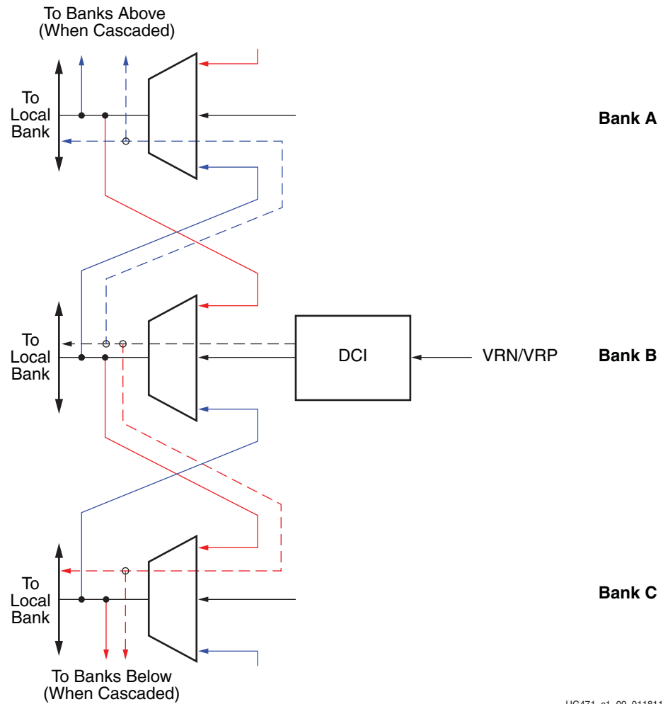
Figure 1-7: DCI Cascading Supported Over Multiple I/O Banks
